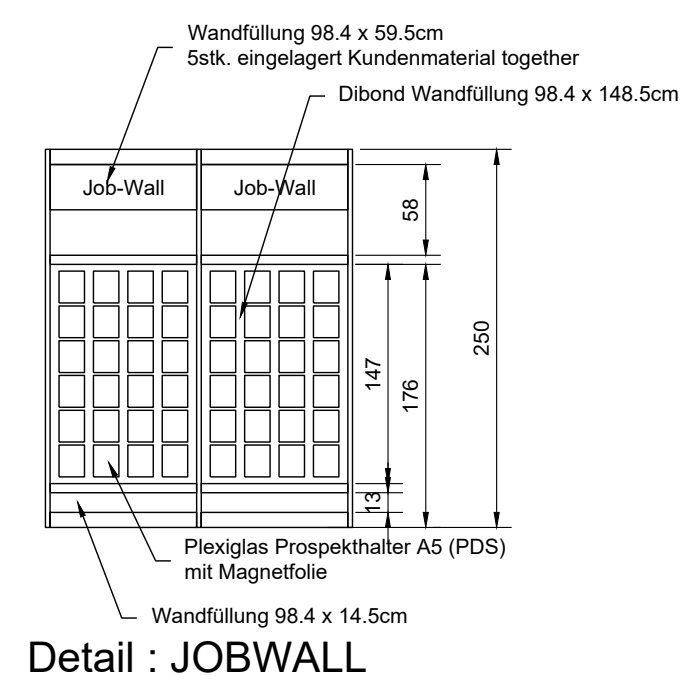
Detail : JOBWALL
